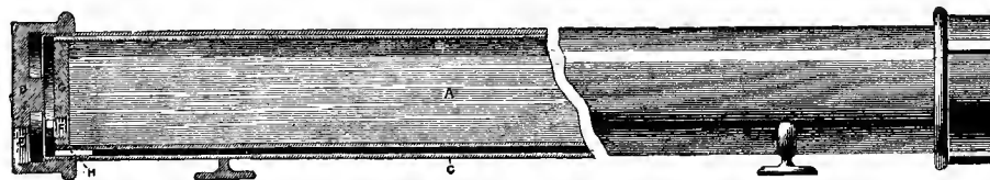
Fig. 3009 Sectional Elevation. GOLD'S STORAGE HEATER (Iron).
